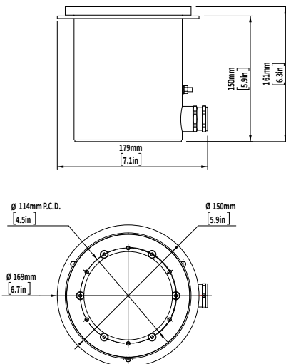
FAIELN - Liner pool installation housing
