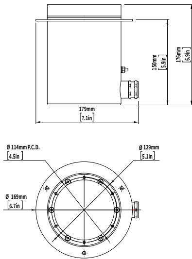
FAIE - Concrete pool installation housing side feed
