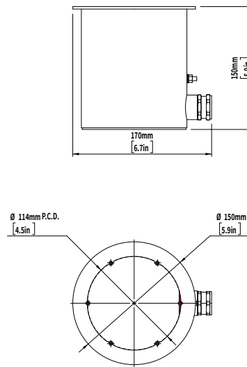
FAIESP - Stainless steel pool installation housing
