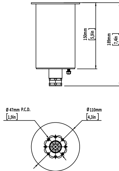
FAM382SP - Stainless Steel Pool Installation
