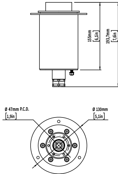
FAM382 - Concrete Pool Installation back feed
