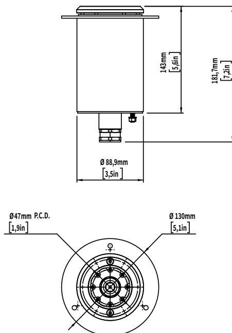
FAM382LN - Liner Pool Installation
