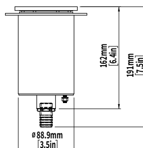
AM382LN - Liner Pool Installation
