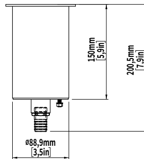
AM382SP - Stainless Steel Pool Installation
